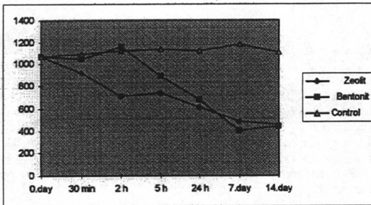
Figure 2 Concentration of ammonia in mg/l in pig slurry treated with zeolite Z (50 g.l -1 ) and bentonite B (50 g.l -1 ) in dependence on the time of contact in comparison with the control (K).
