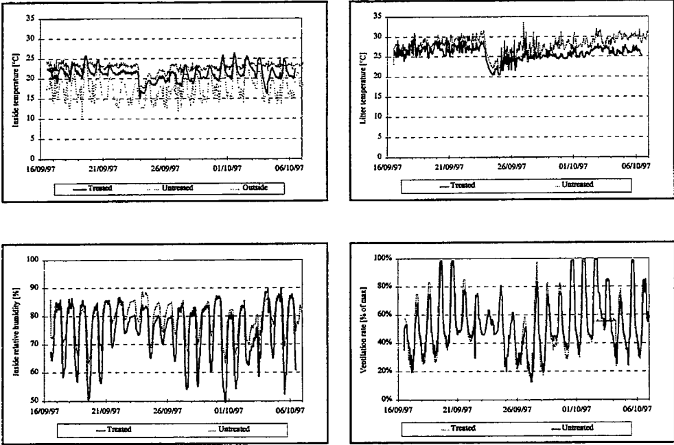
Figure 2 Monitoring data trend during second experimental period: outside, inside and litter temperature, inside relative humidity and ventilation rate.
