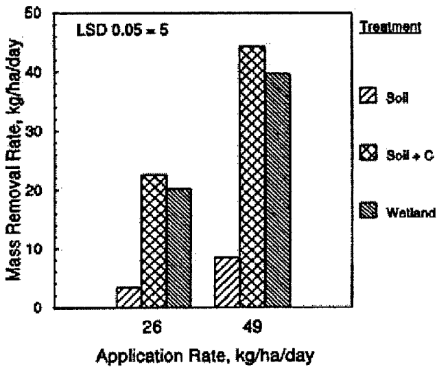
Figure 3 Nitrogen removal from wetlands microcosms with three types of carbon regimes and batch wastewater applications every four days.
