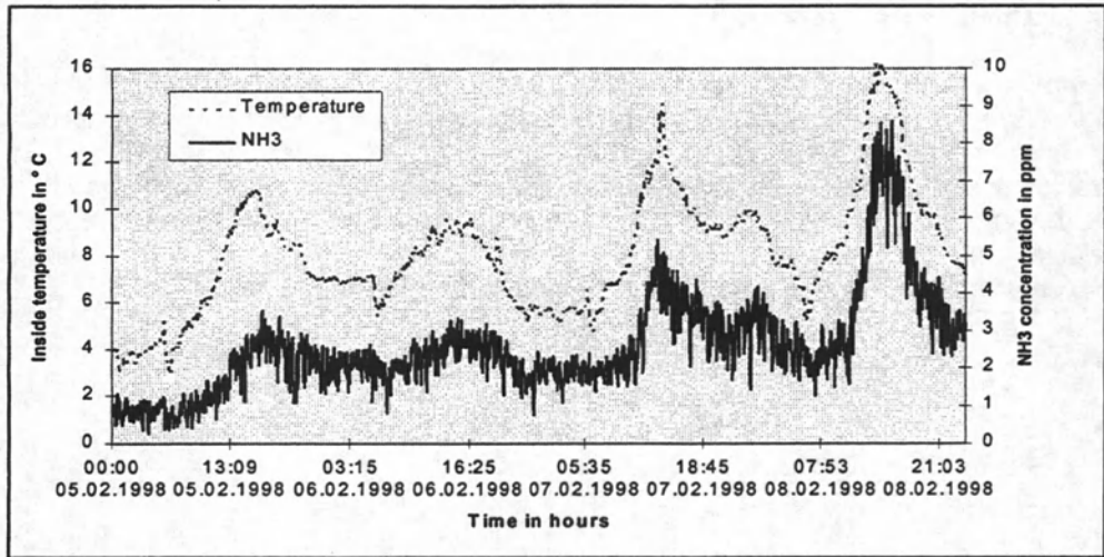
Figure 1 Temperature influence on ammonia concentration in condition without wind
