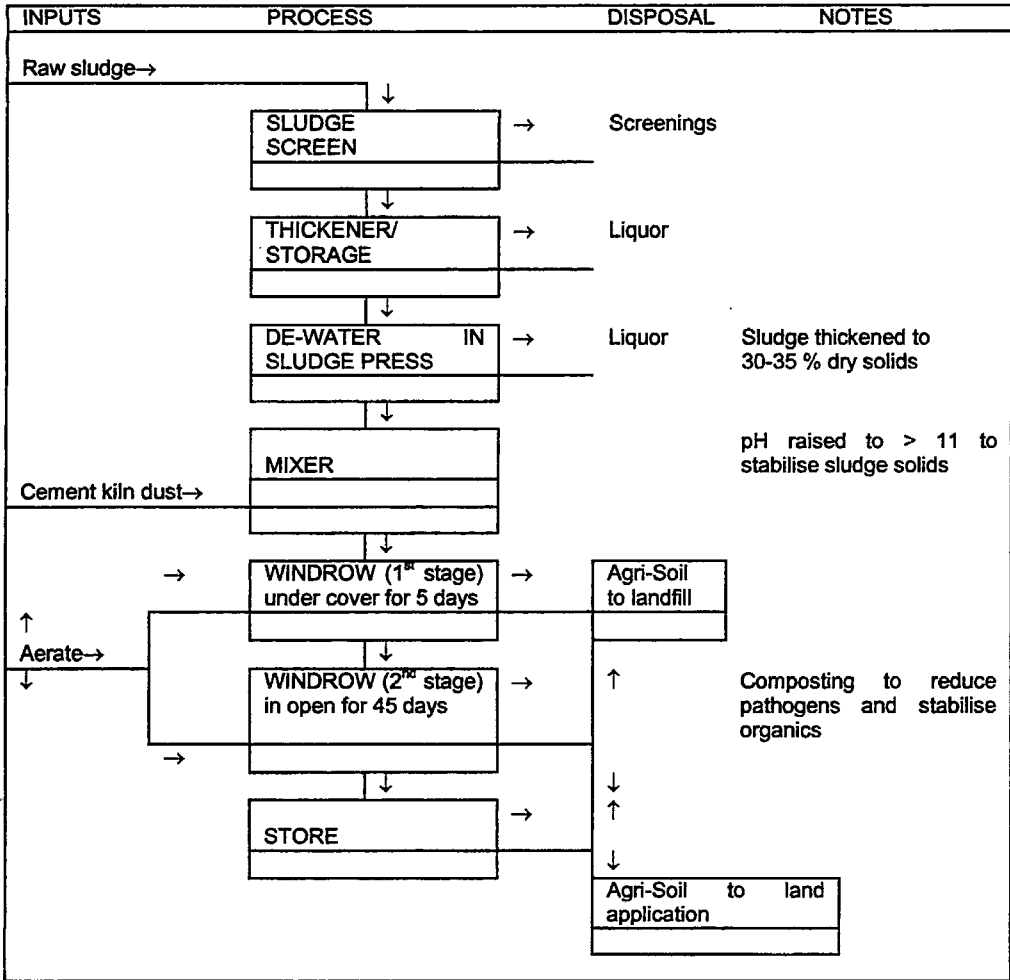
Figure 1 Agri-Soil process flow diagram
