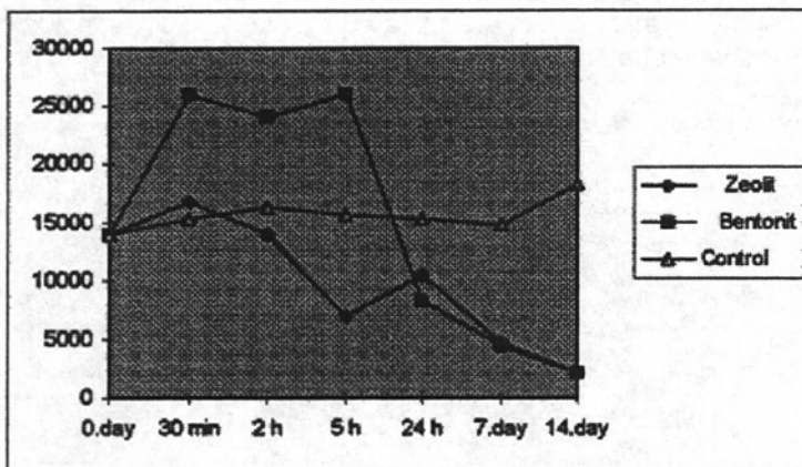
Figure 3 Concentration of chemical oxygen demand in mg/l in pig slurry treated with zeolite Z (50 g.l -1 ) and bentonite B (50 g.l -1 ) in dependence on the time of contact in comparison with the control (K).
