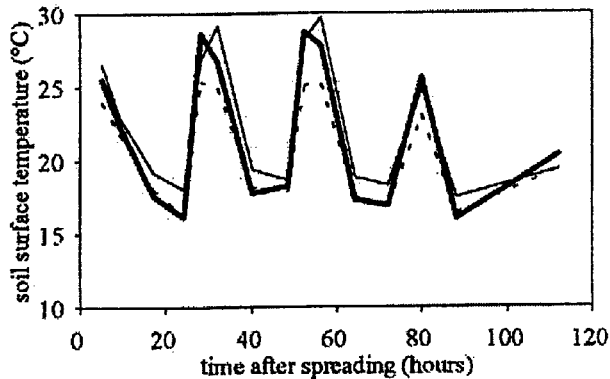
Figure 2 Variations in soil surface temperature obtained in Exp. 7, using either a sunshade (broken line) or a heating resistance (thin line) compared to the reference treatment (thick line).
